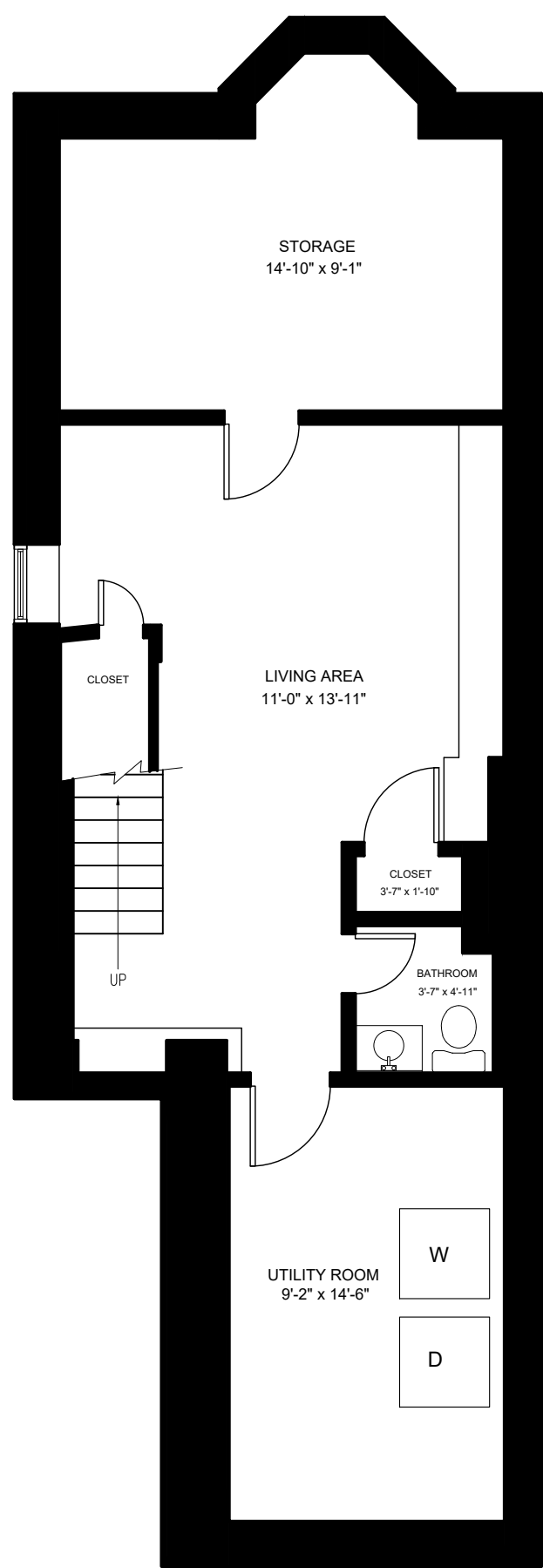
BASEMENT
