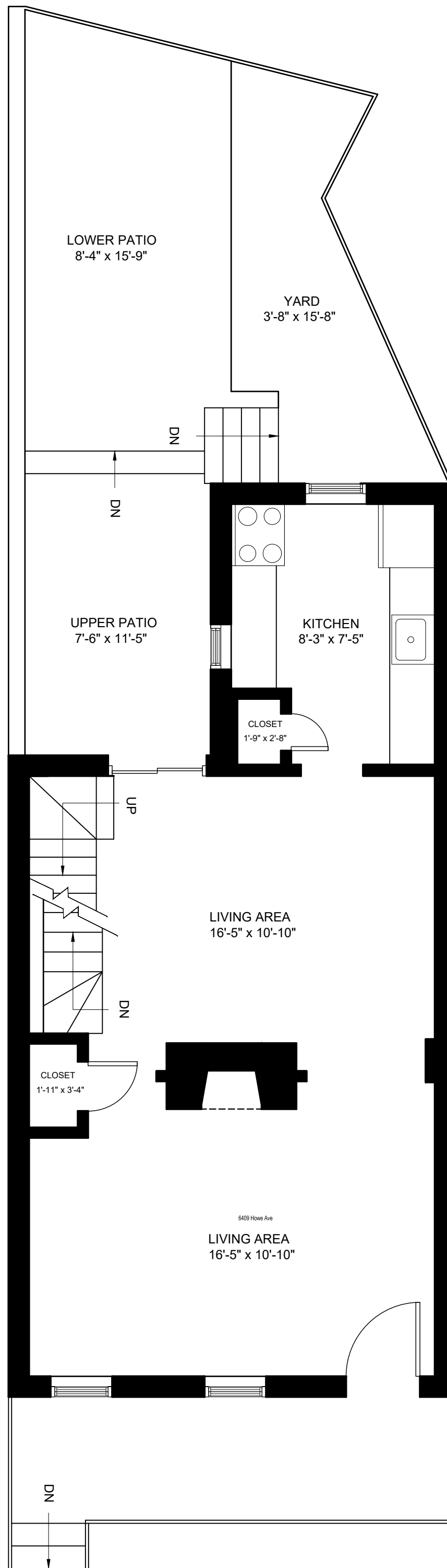
FIRST FLOOR
